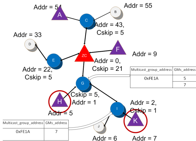
Fig. 4. An example of updating the multicast table
